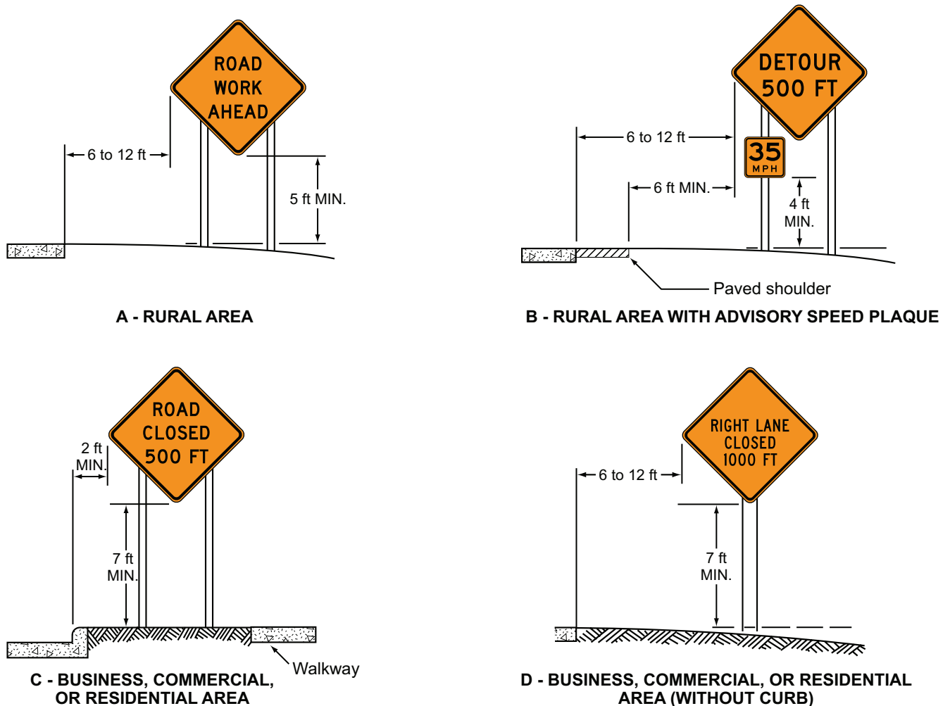
Figure 6F-1. Height and Lateral Location of Signs on Posts—Typical Installations
